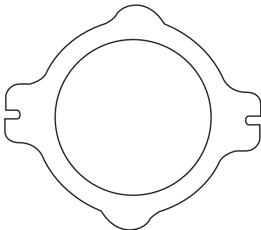
669 ø 87.20 x 65.5 x 1 mm
