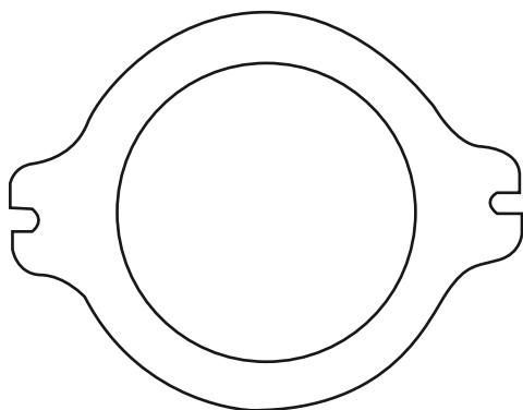
607 Bristol 10 - 15 - 20 HP 48 x 36.5 x 62 x 04 mm
